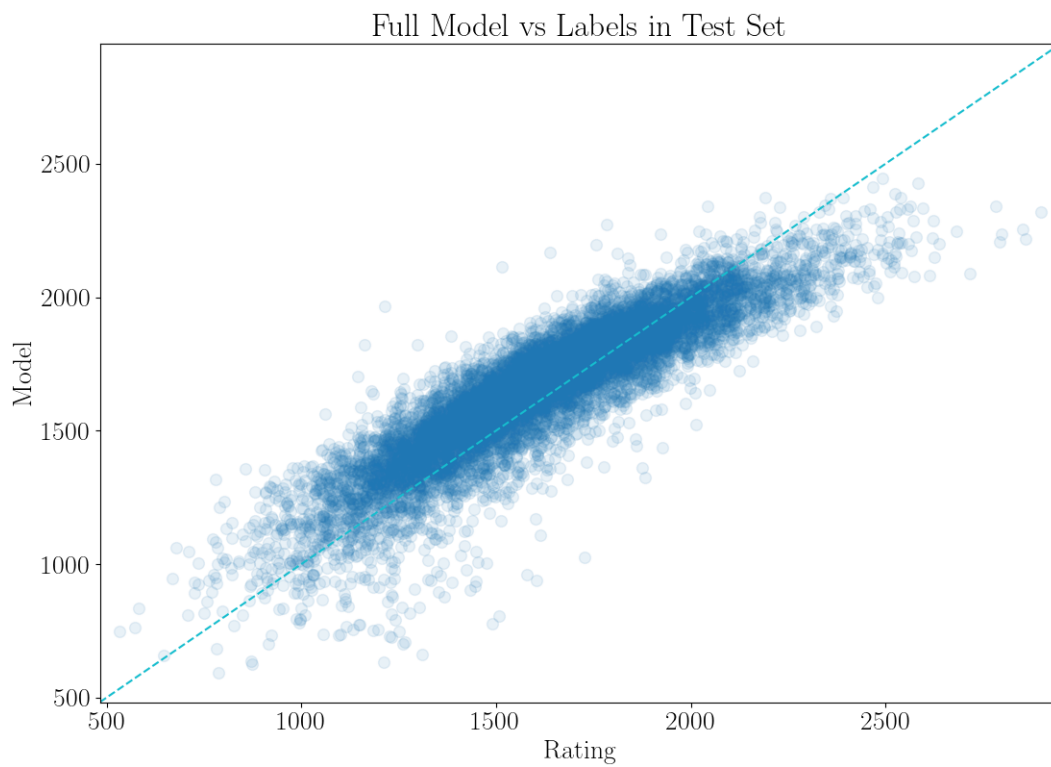
Figure 5.8: In this figure, we compare the rating determined by our full model before every game with the associated label. It shows that the model tends to err towards the mean, just like Glicko-2 does.
