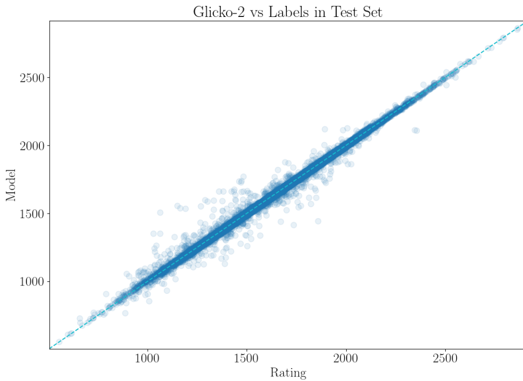
Figure 5.6: In this figure, we compare the rating determined by Glicko-2 before every game with the associated label. It shows that Glicko-2 tends to slightly err towards the mean. Because the labels are the Glicko-2 ratings of the same players from the future, we interpret the off marks as instances where the players' rating has not yet settled in the system.
